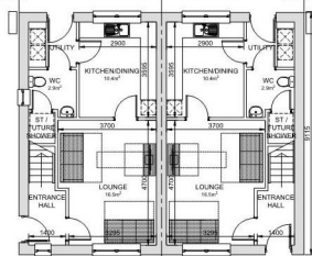
GROUND FLOOR PLAN 3 BED VILLA
